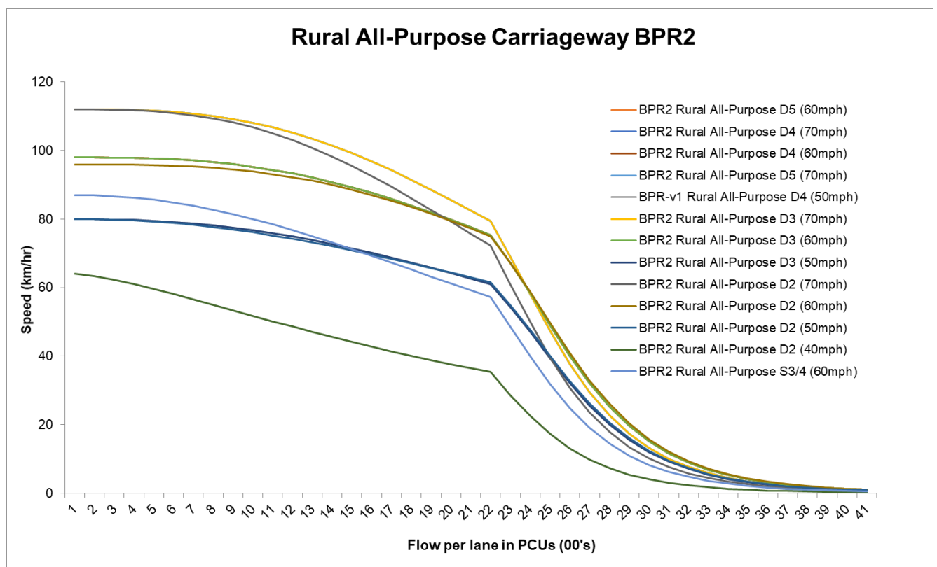
Figure 6-2: VDF Rural All-Purpose Carriageway Link Type
