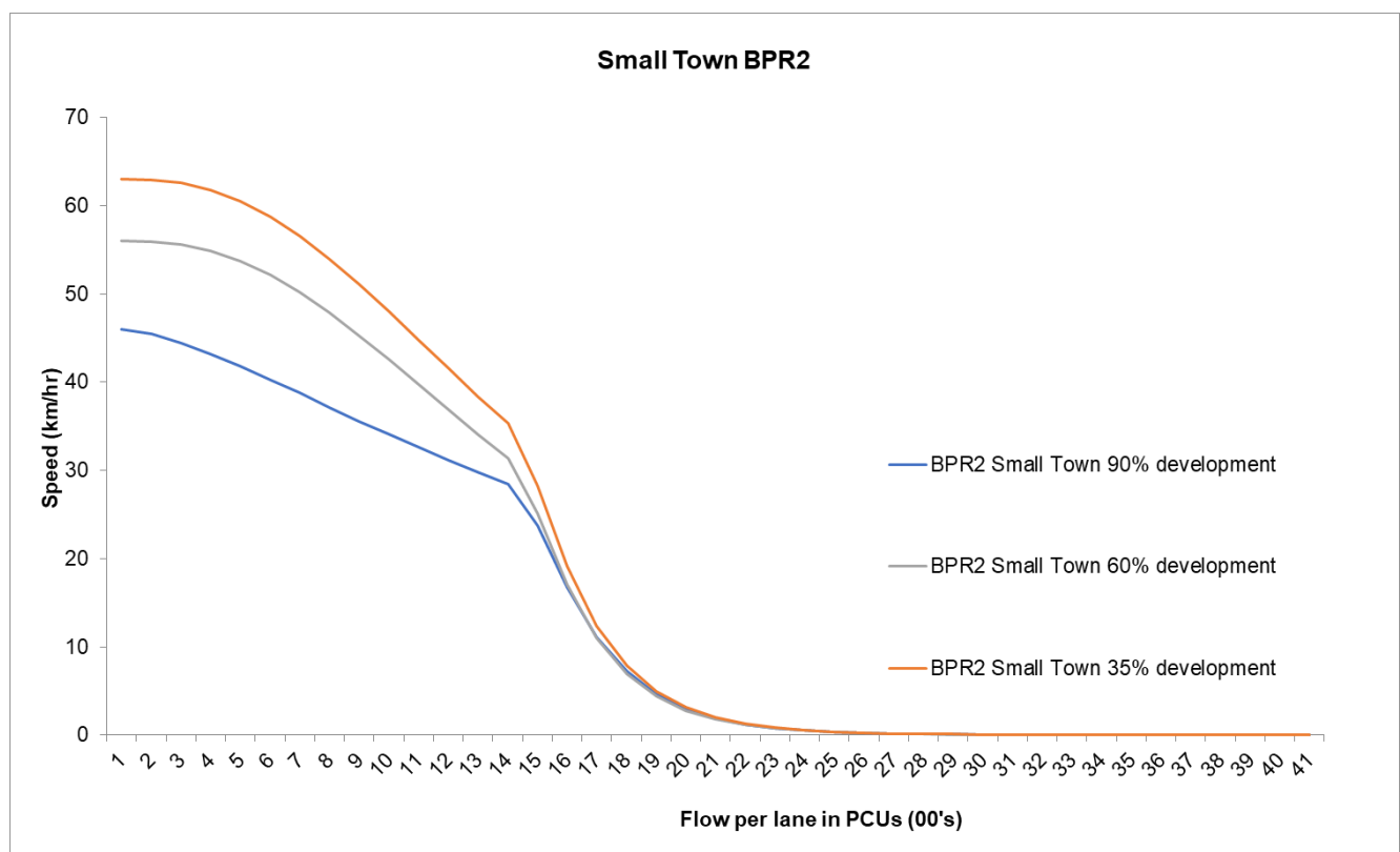
Figure 6-6: VDF Small Town Link Type
