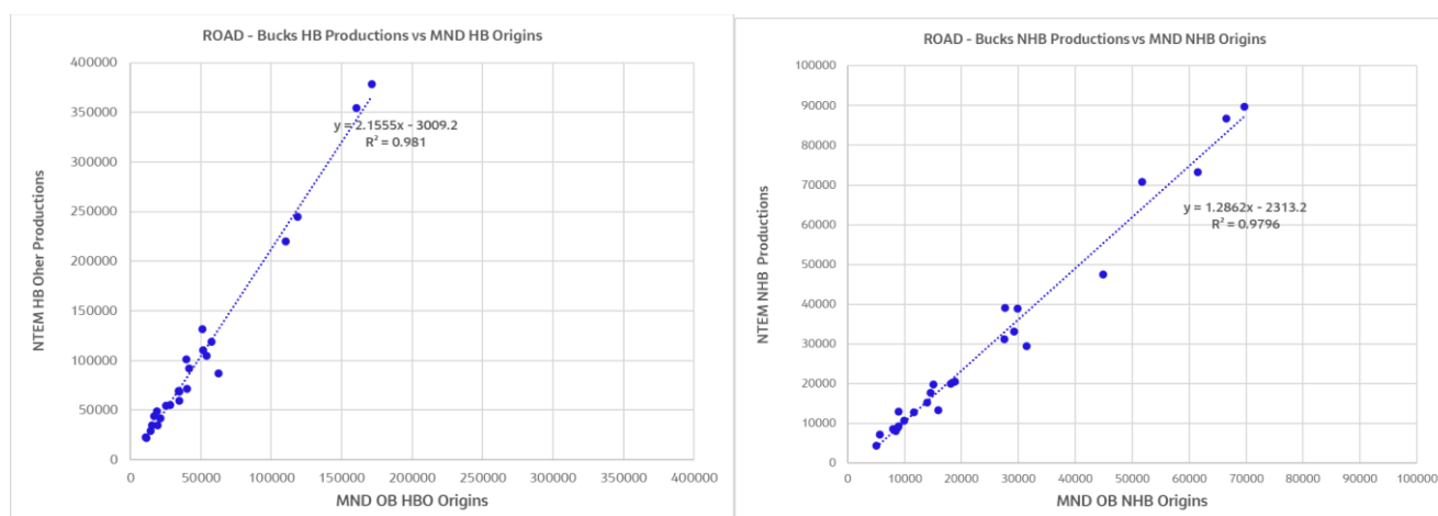
Figure 9-6: Sector Comparison of MND and Synthetic NTEM Trip Ends – Productions
